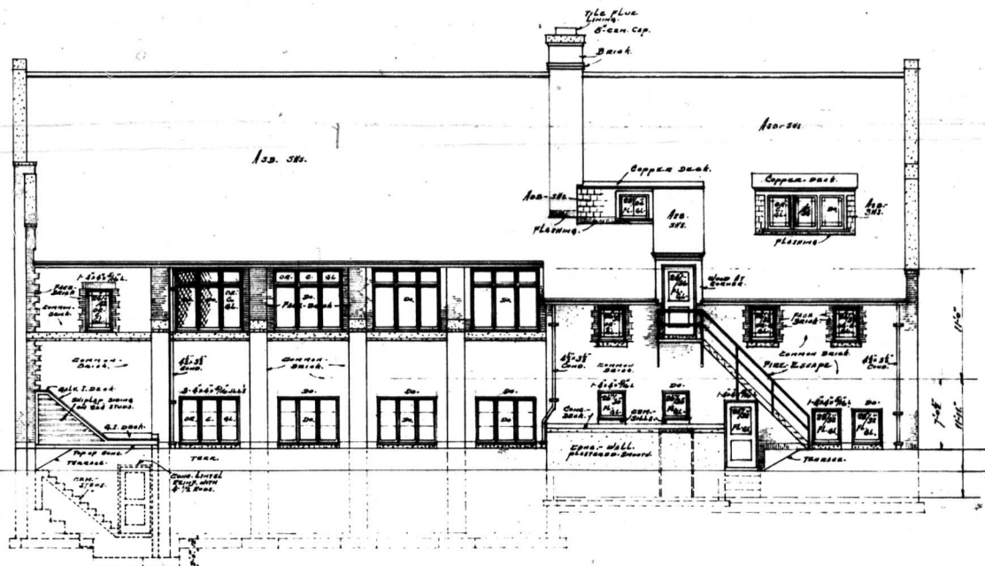
WEST - ELEVATION. 1/8" scale.
