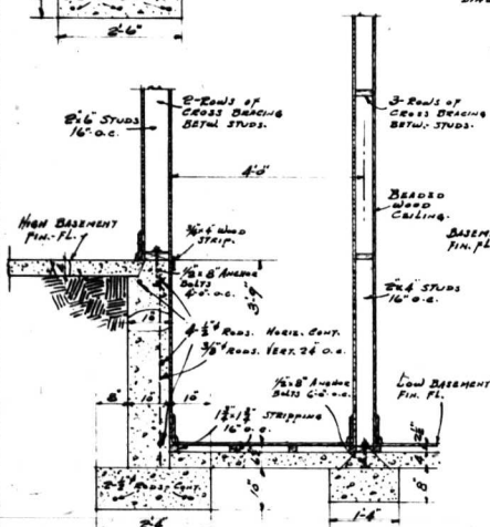
CONCRETE RETAINING WALL BETW. HIGH & LOW BASEMENT. 1/8" SCALE.
