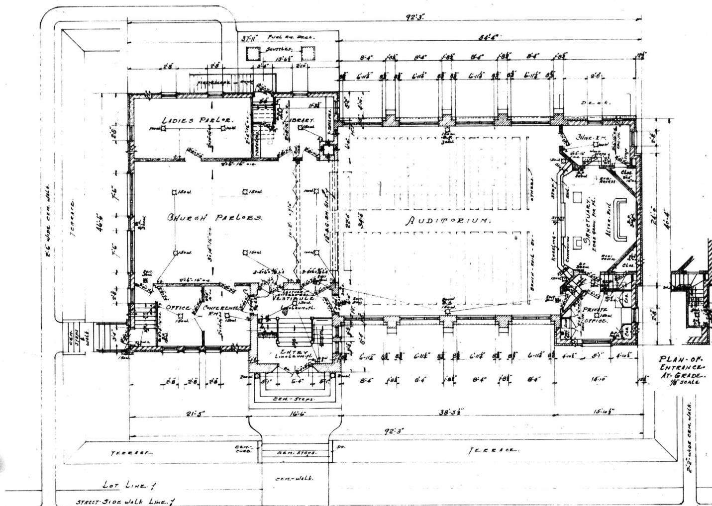
FIRST FLOOR PLAN. 1/8" SCALE.
