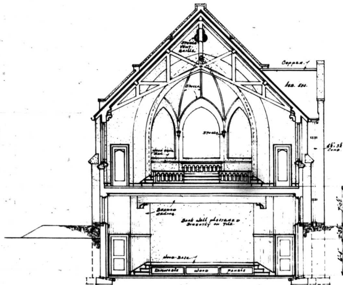
TRANSVERSE SECTION. TOWARD SANCTUARY. 1/8" scale.
