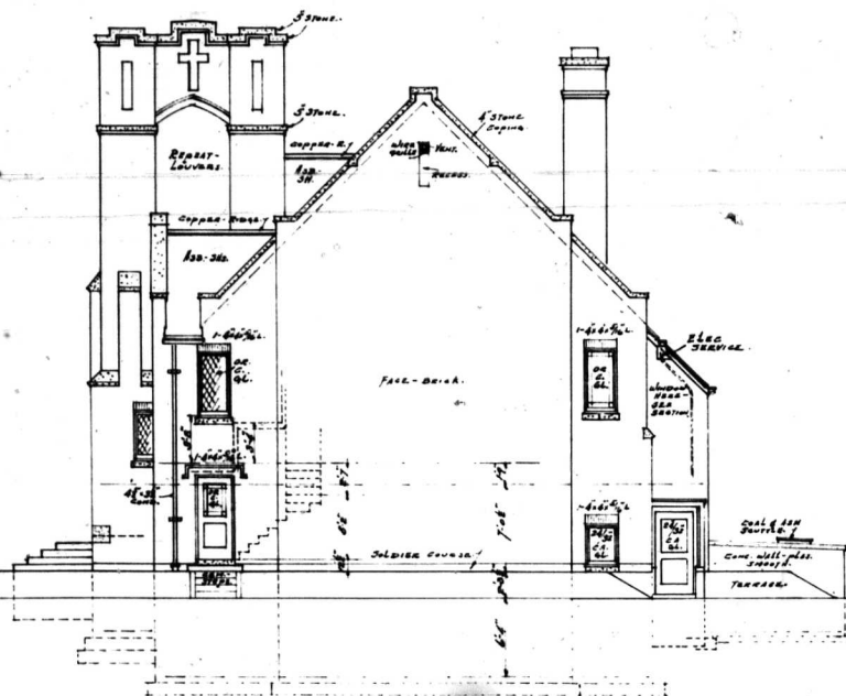
NORTH - ELEVATION 1/8" scale.
