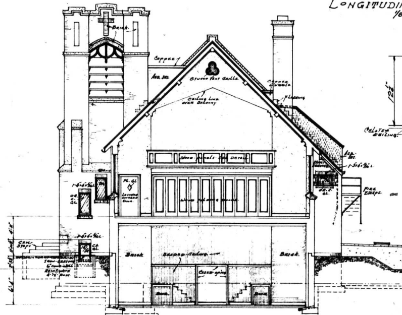
TRANSVERSE SECTION TOWARD BALCONY. 1/8" scale.
