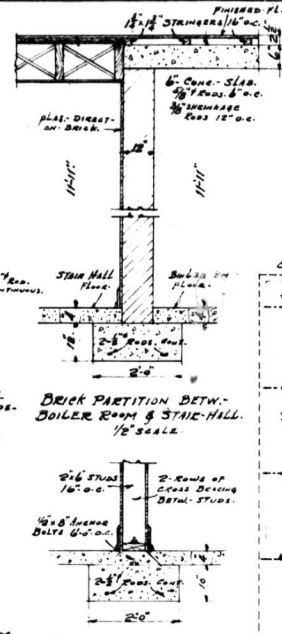
CONCRETE FOOTING FOR FRAME-LOAD BEARING WALL. 1/8" SCALE.
