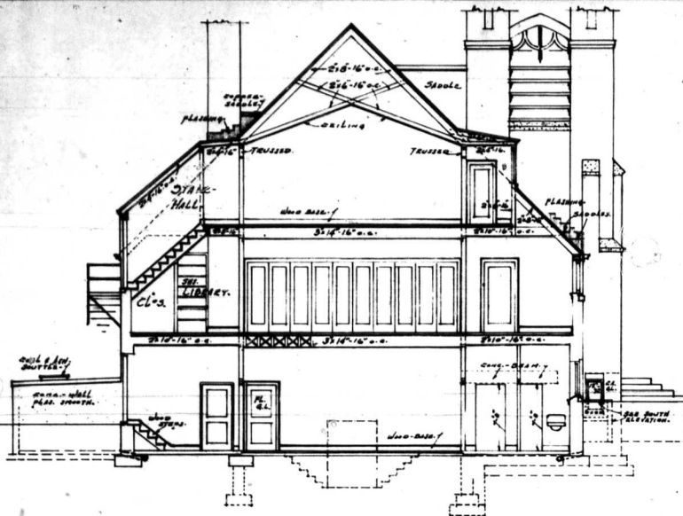
TRANSVERSE SECTION - THRU CHURCH PARLORS 1/8" scale.
