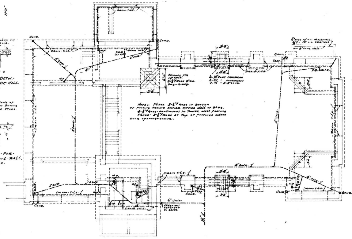
FOUNDATION & SEWERAGE PLAN. 1/8" SCALE.
