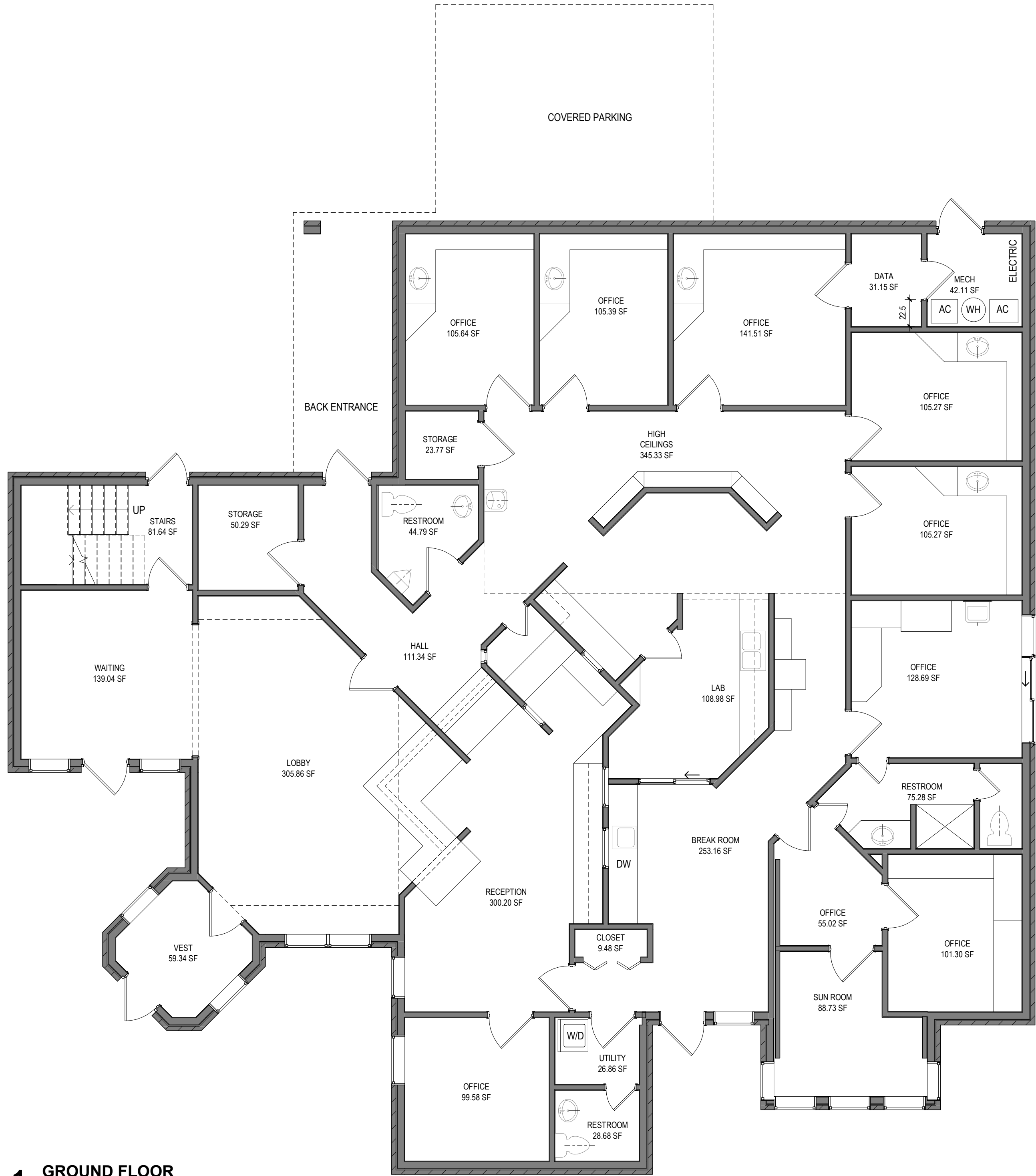
1 GROUND FLOOR SCALE: 3/16" = 1'-0"
