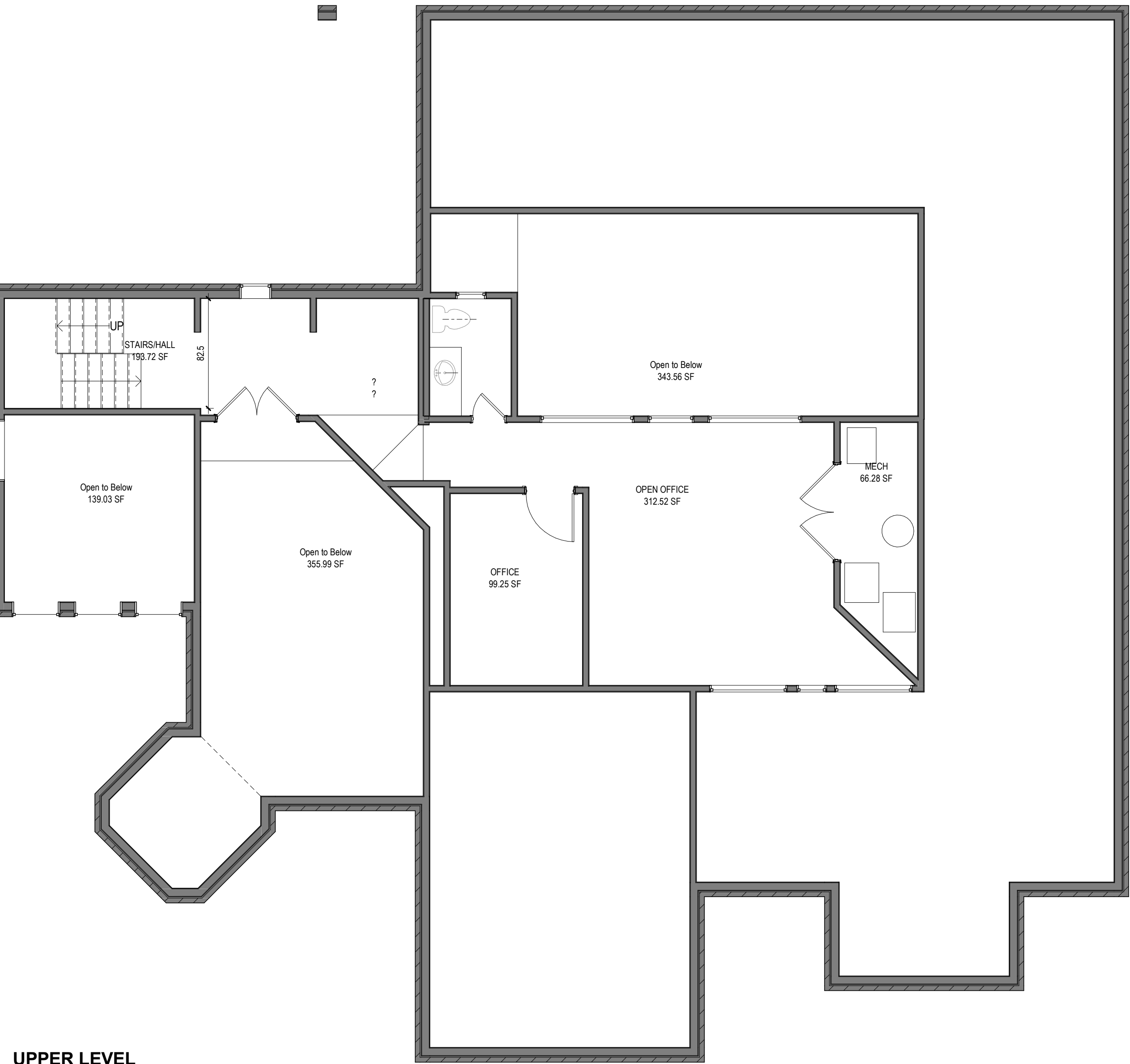
2 UPPER LEVEL SCALE: 3/16" = 1'-0"
