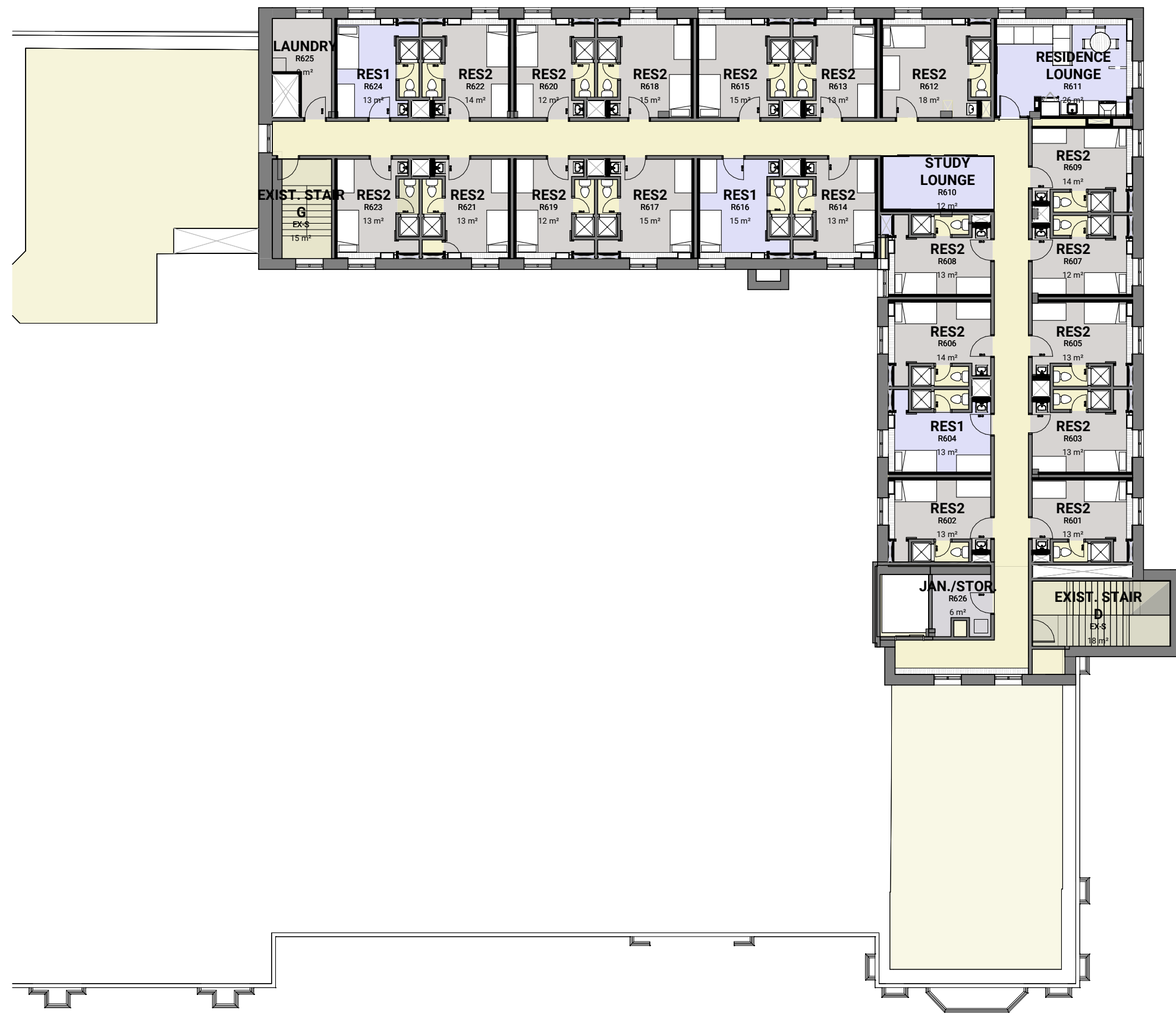
JDUC EXISTING OVERALL PLAN RESIDENCE RENOVATION- EXIST. LEVEL 6 3 A4.02 1:200
