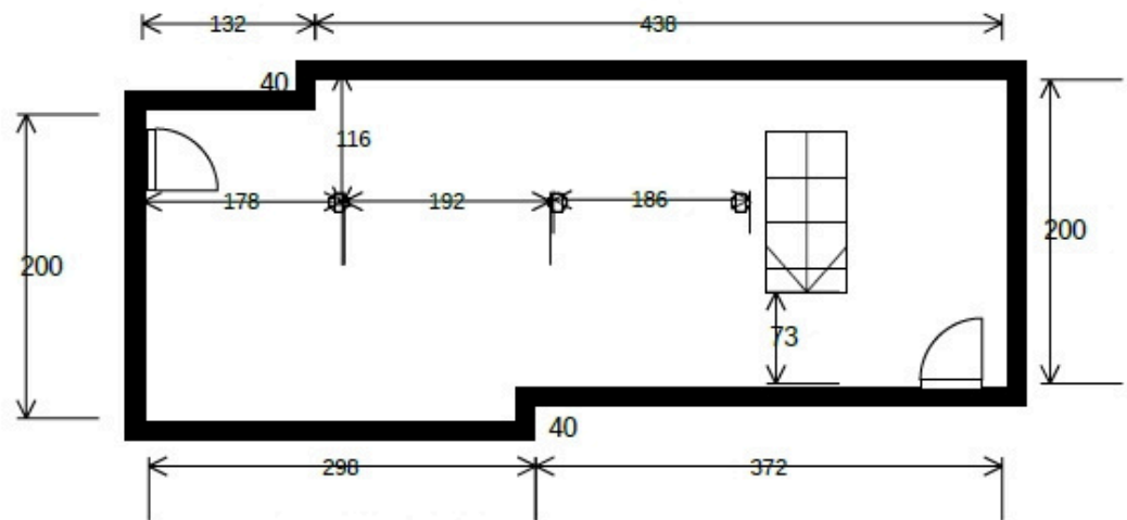
LOWER LEVEL
