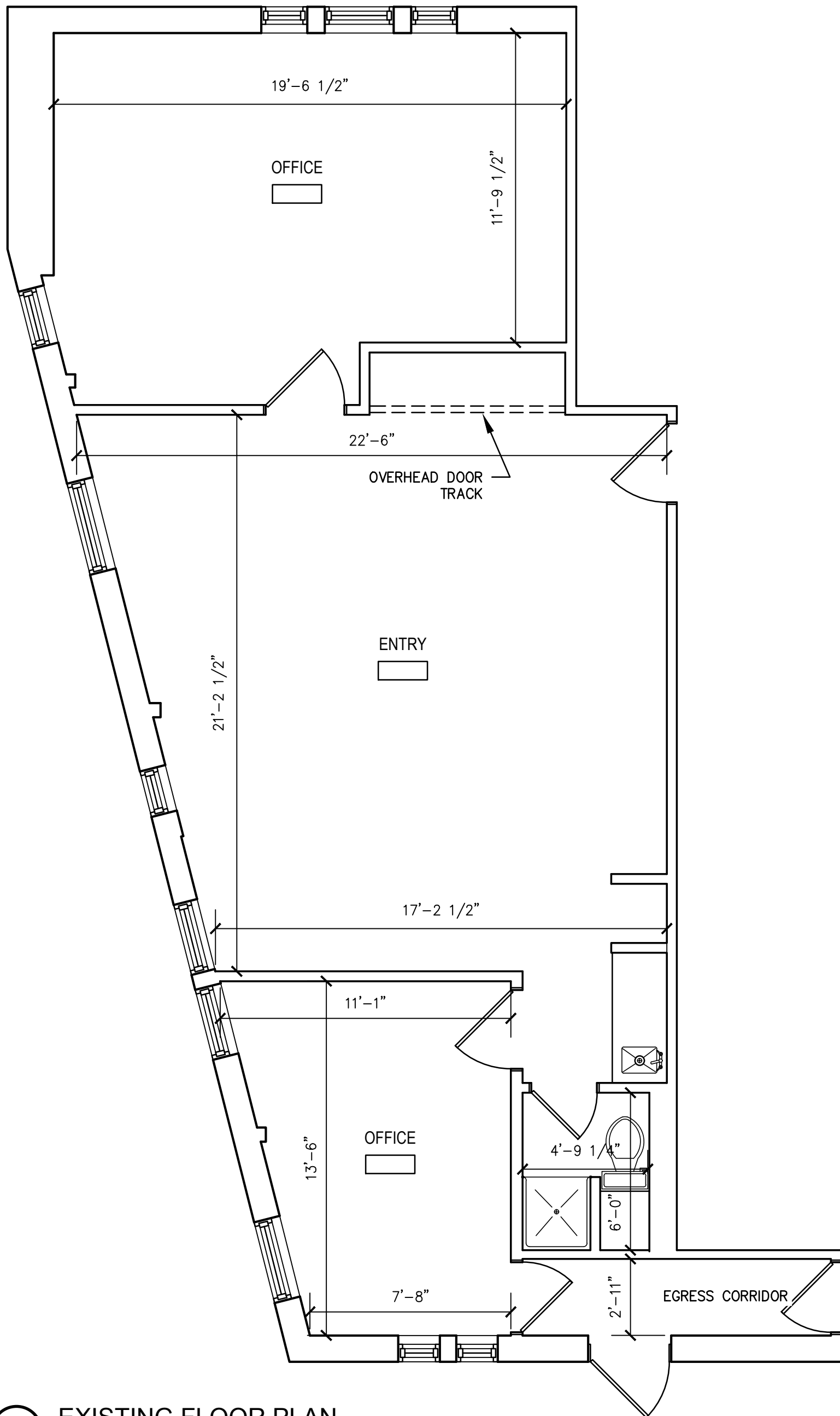
1 EXISTING FLOOR PLAN 1/4" = 1'-0"
