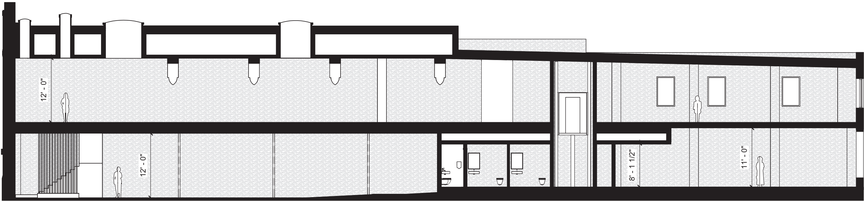
BUILDING SECTION
