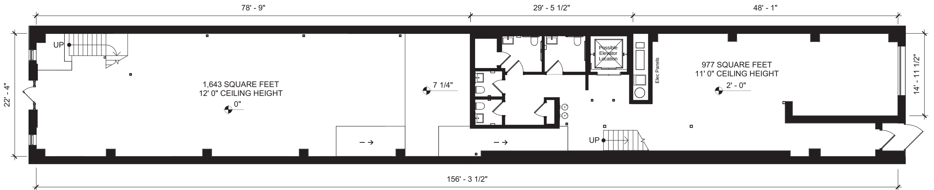
FIRST FLOOR
