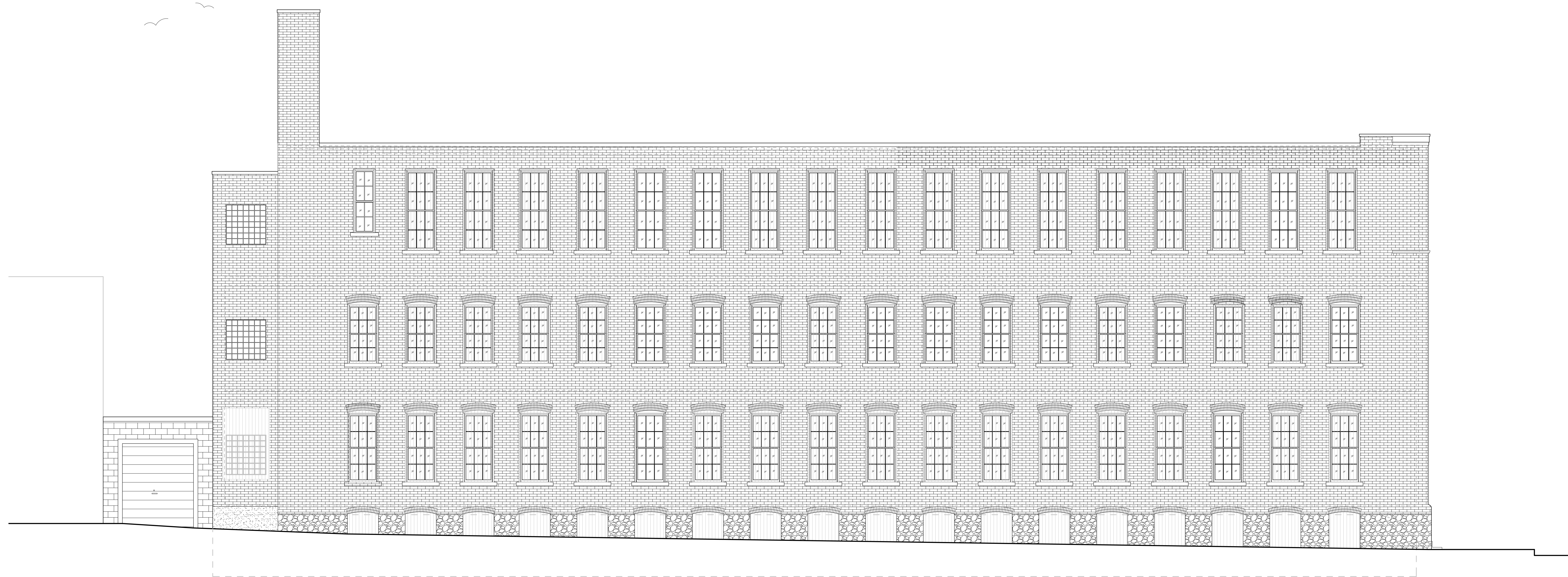
SOUTH ELEVATION 53 CANAL STREET
