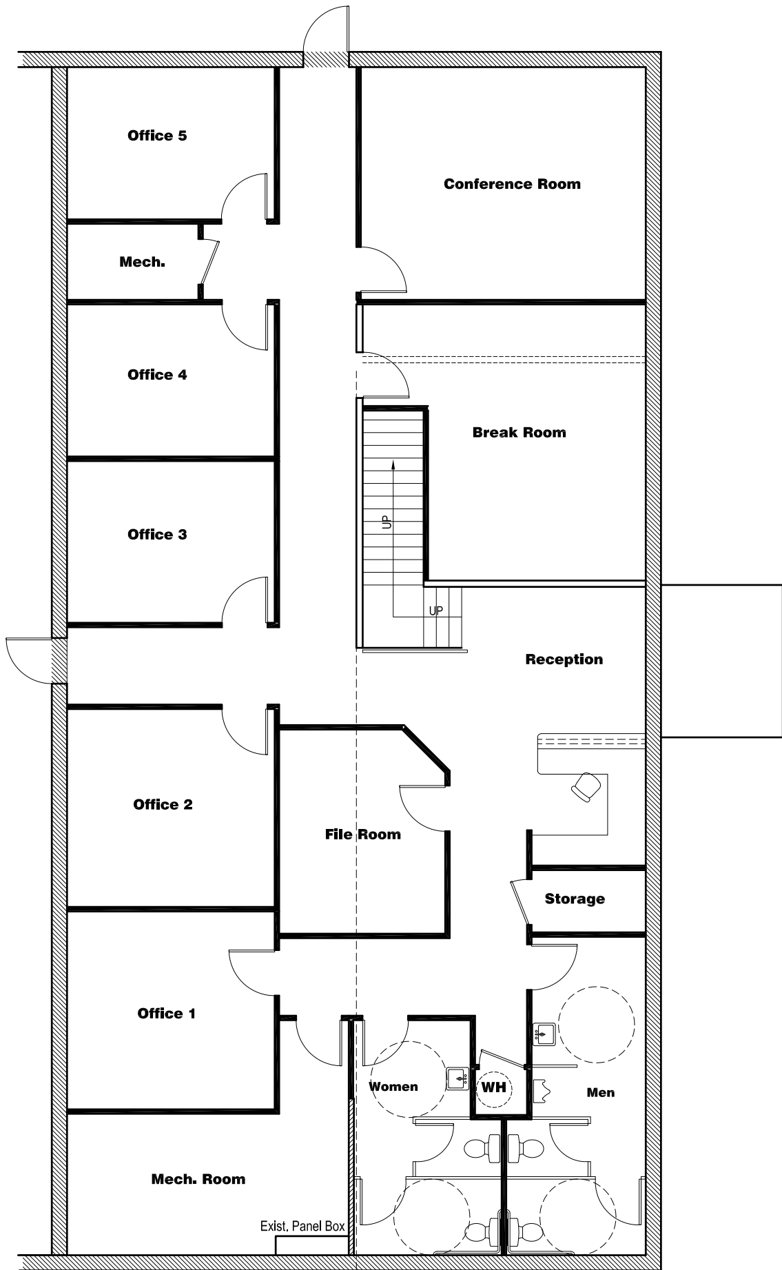
MAIN FLOOR PLAN OFFICE REMODEL EXIST. BLDG.
