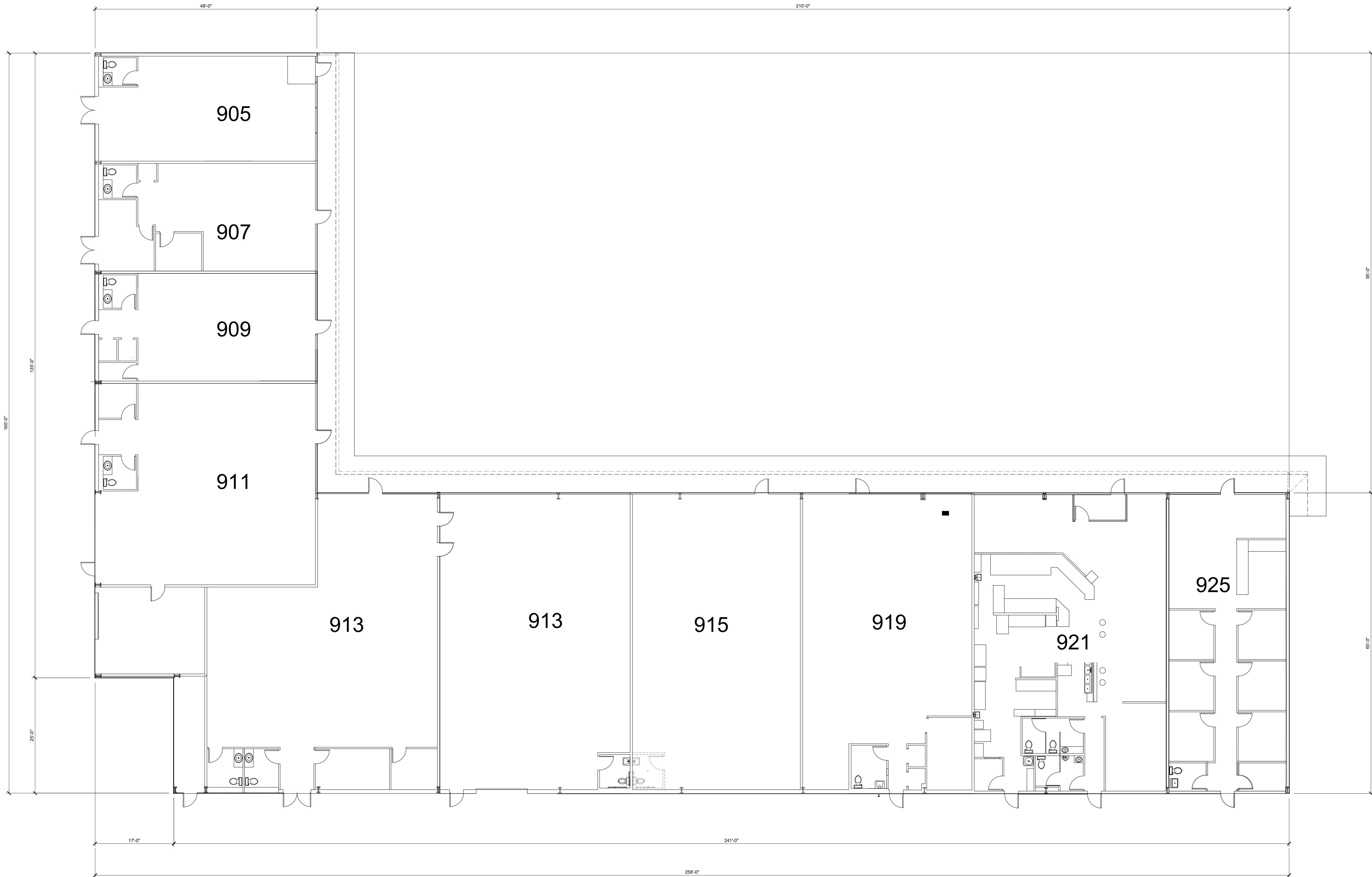
1 A-100 SCALE 1" = 10' 20,905 Sq. Ft. GENERAL BUILDING PLAN
