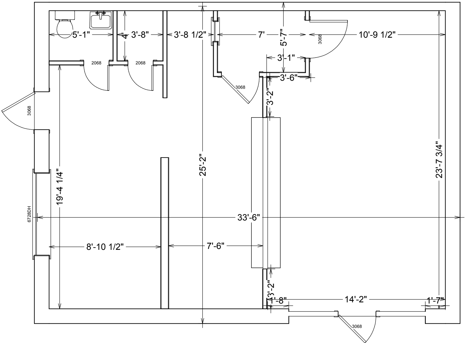
150 N 11th Approximately 843 sq. ft. Based BOMA Standards Ceiling Height 8' 10"
