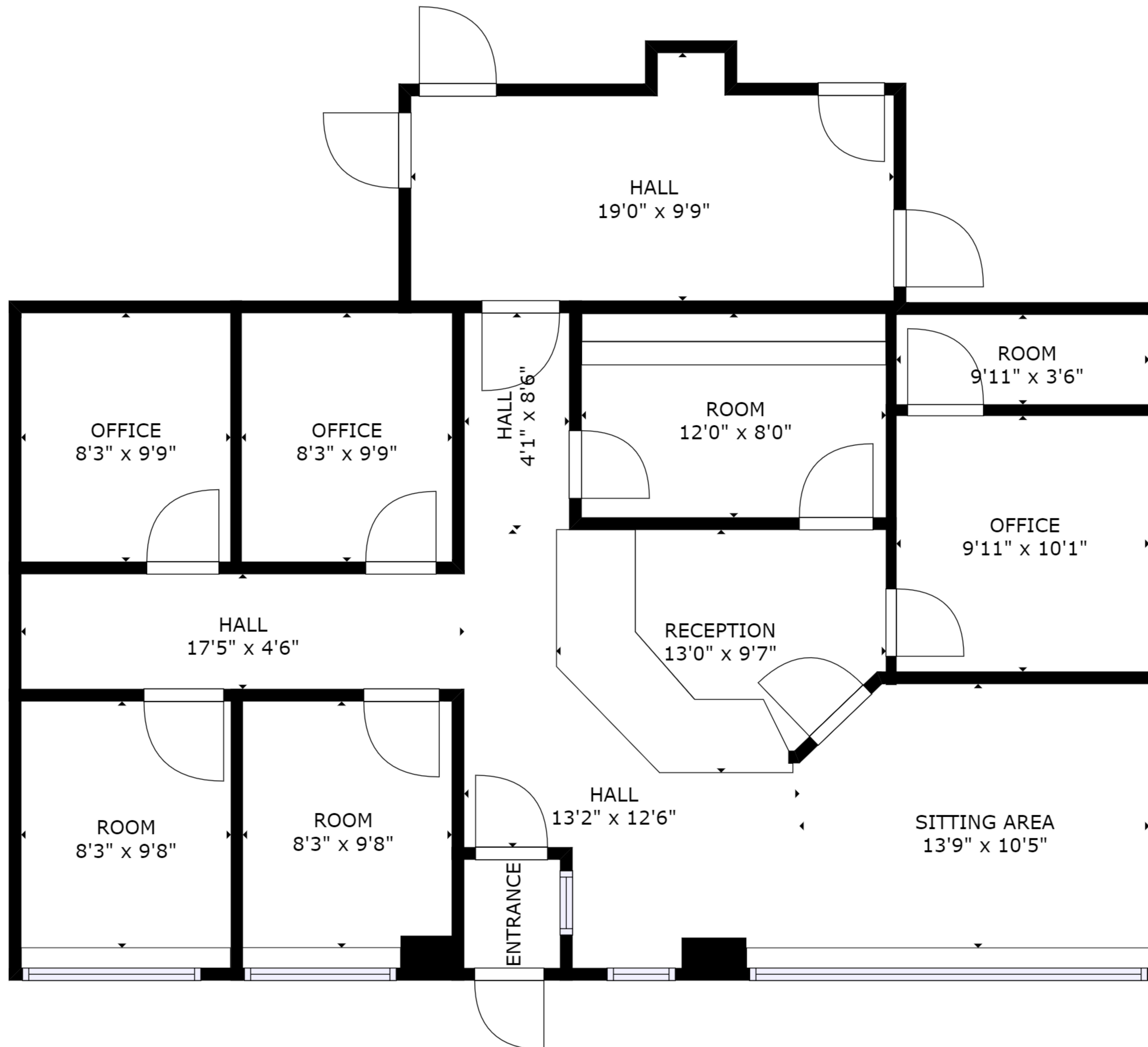
FLOOR 1
