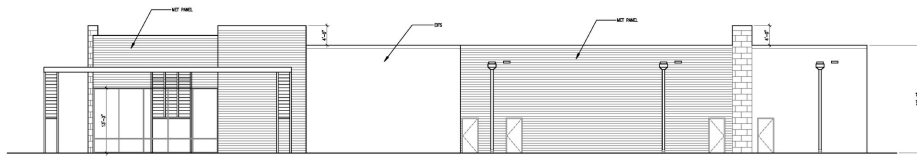
WEST ELEVATION
