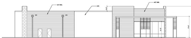
SOUTH ELEVATION
