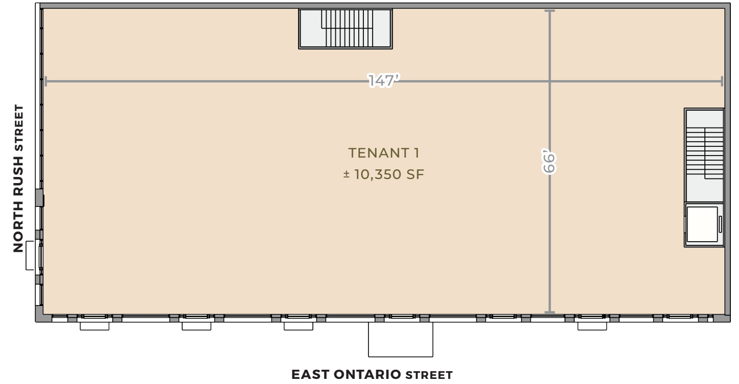
Second Floor
