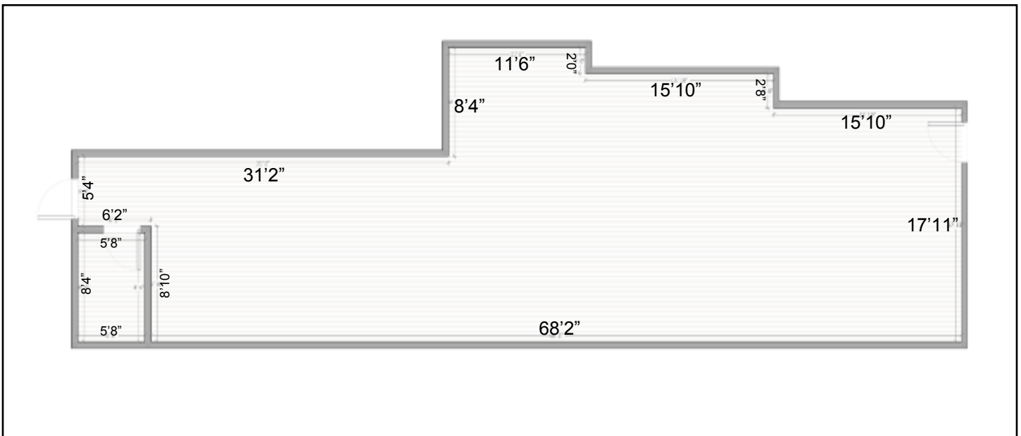
Floor Plan
