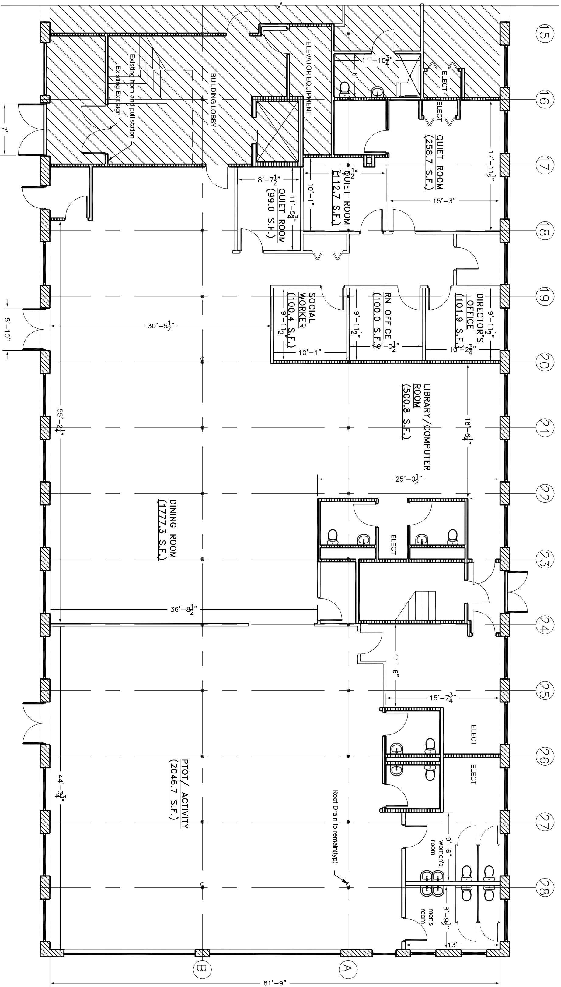
First Floor Napping Building Partial Plan Scale 1/8" = 1'-0"
