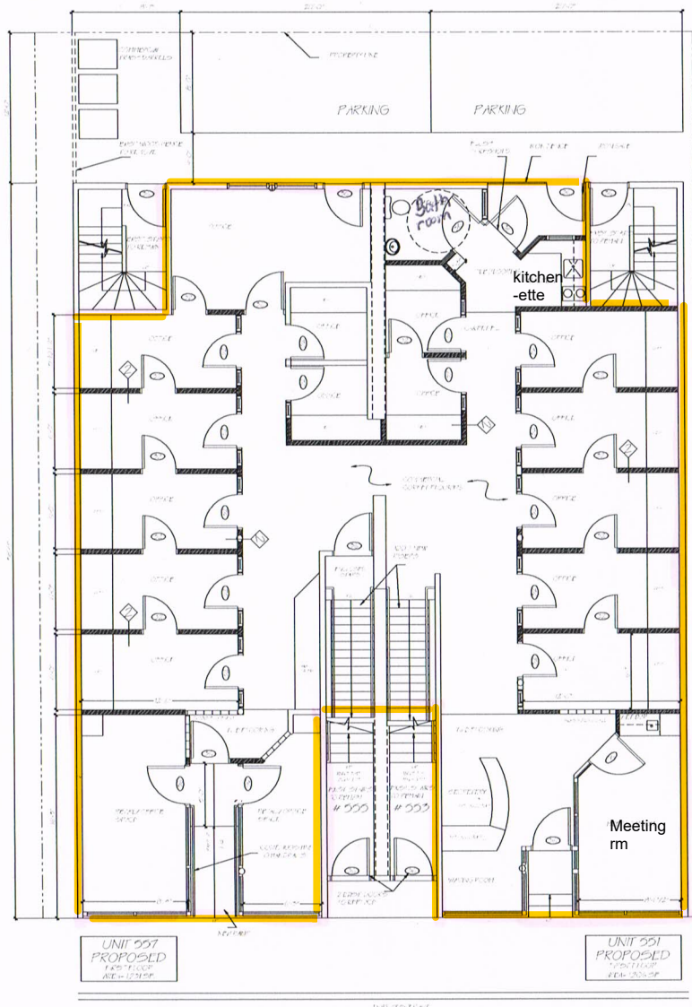
② PROPOSED FIRST FLR. PLAN SCALE: 1/4" = 1'-0"
