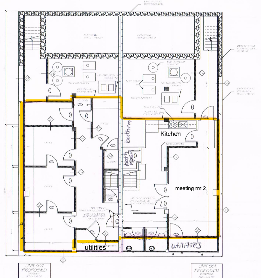
② PROPOSED BASEMENT FLOOR PLAN SCALE: 1/4" = 1'-0"
