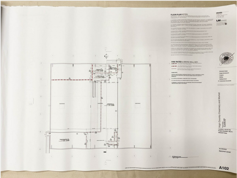
Second Floor Architectural Plan – Approximately 3,738 SF
