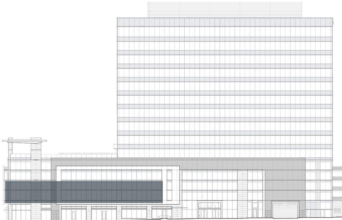
North Elevation
