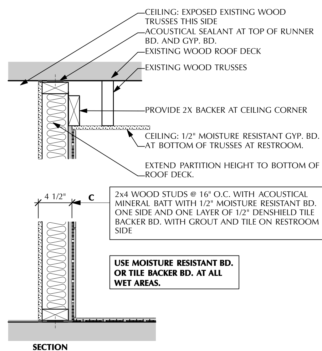
09 Partition Type C Scale: NTS
