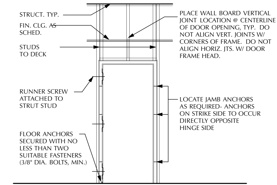
03 Door Framing Detail Scale: NTS
