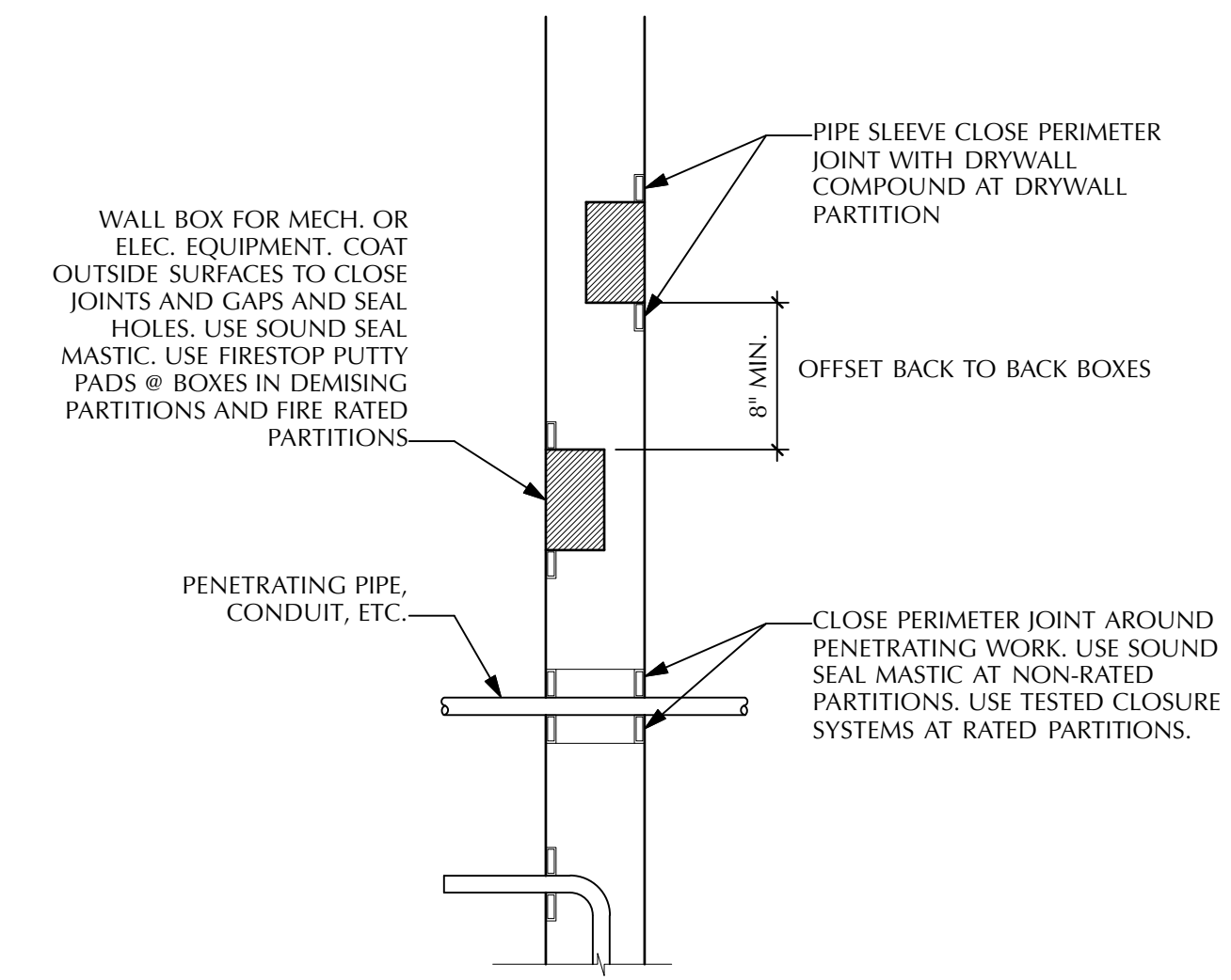
02 Typ. Partition Penetrations Plan Scale: NTS
