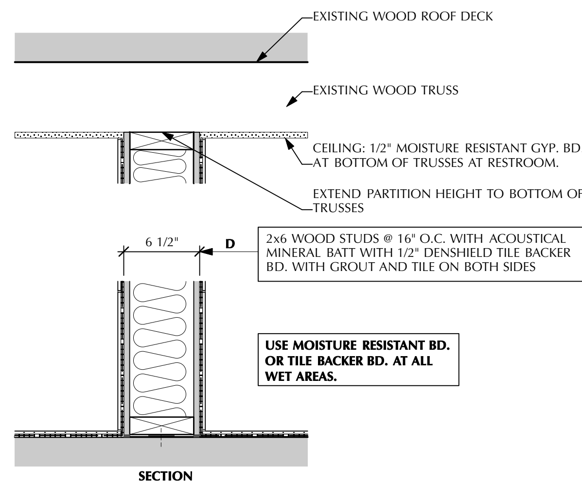
09 Partition Type D Scale: NTS
