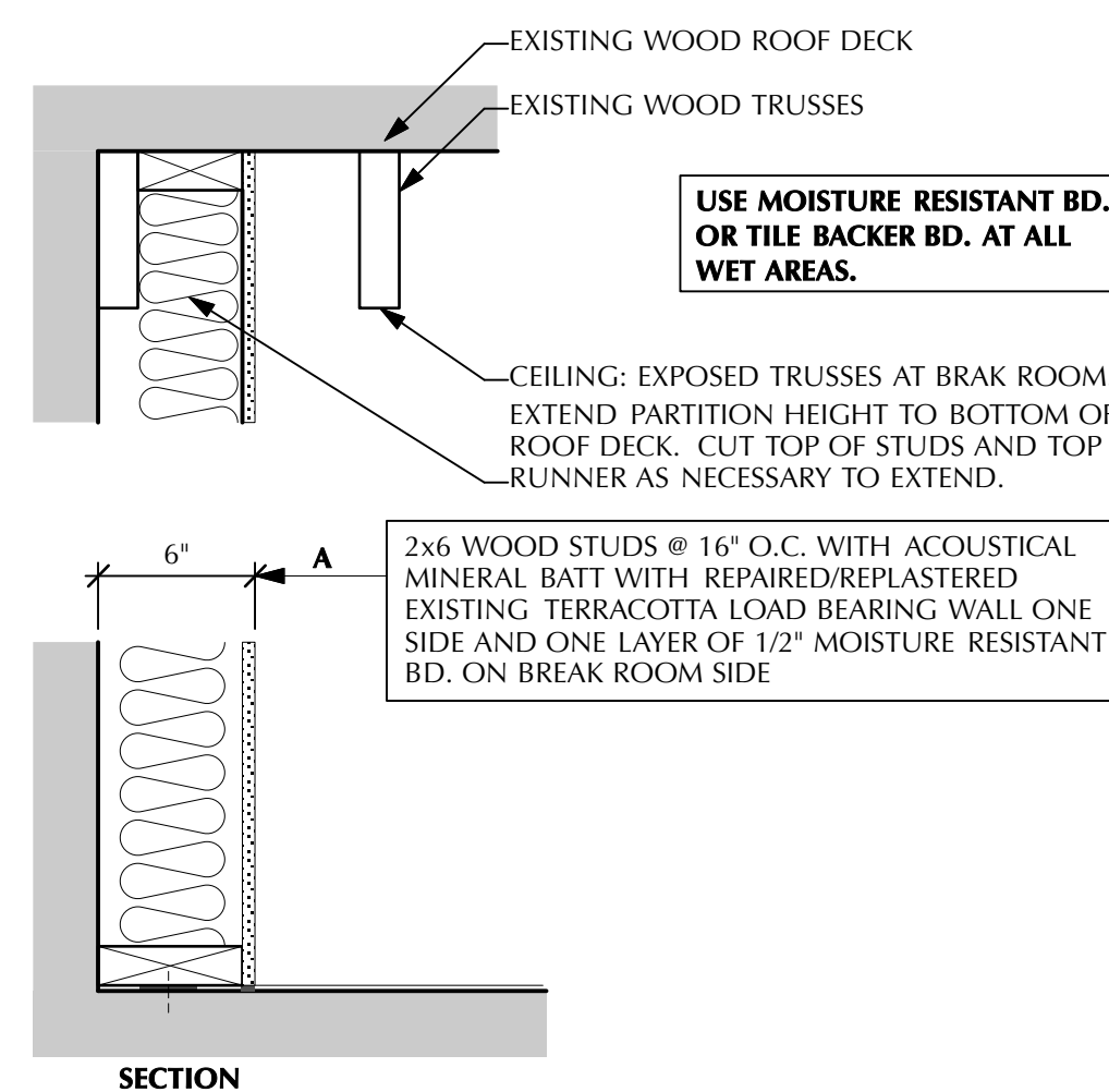
05 Partition Type A Scale: NTS
