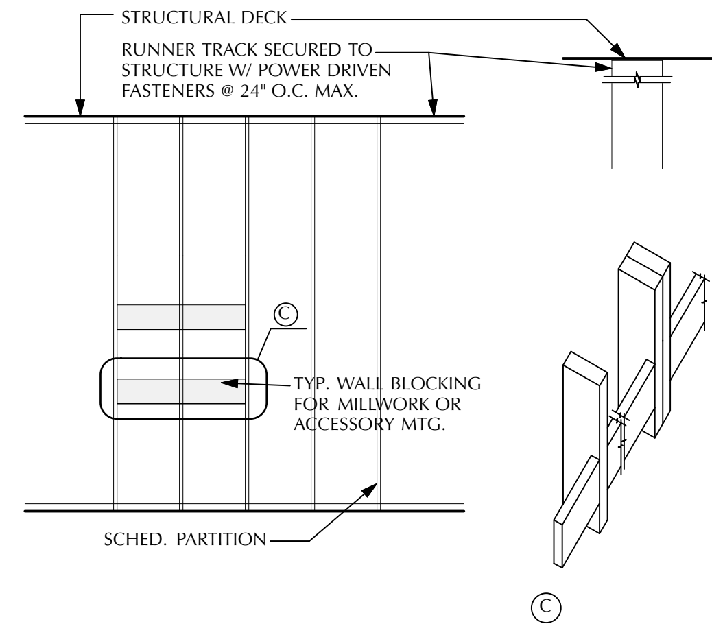
07 Typ. Blocking Detail Scale: NTS
