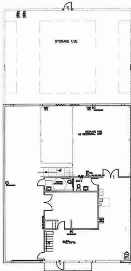
MAIN FLOOR PLAN SCALE: 1/8" = 1'-0"
