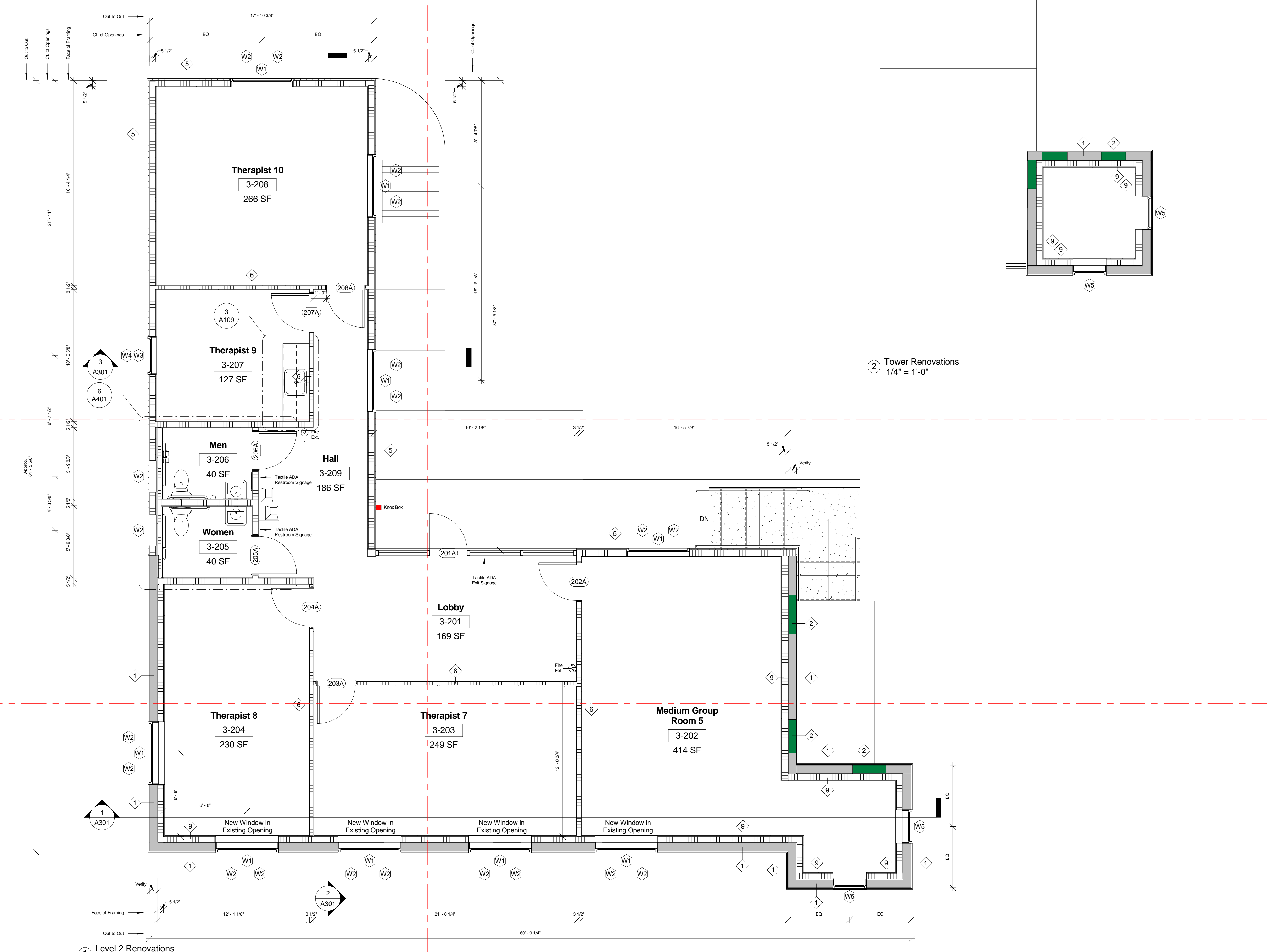
1 Level 2 Renovations 1/4" = 1'-0"
