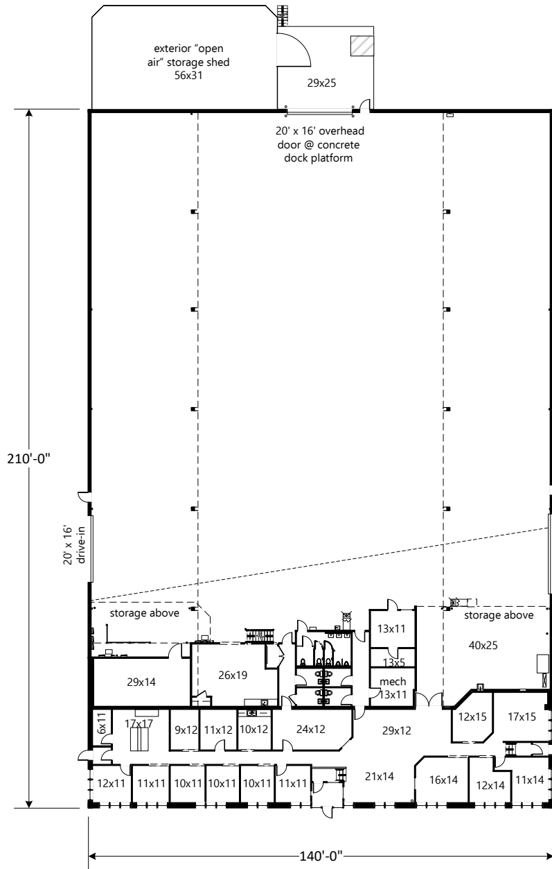
MAIN LEVEL
