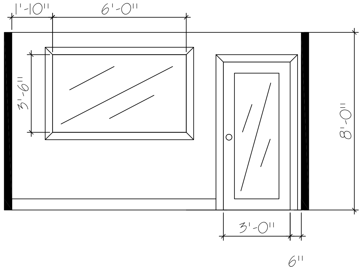
Elevation Conference Room wall w/ Dimensions
