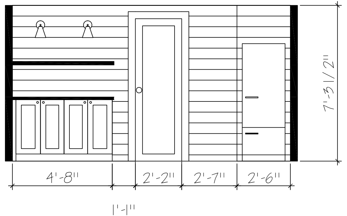
Elevation Lounge Kitchenette wall at Upper Level w/ Dimensions
