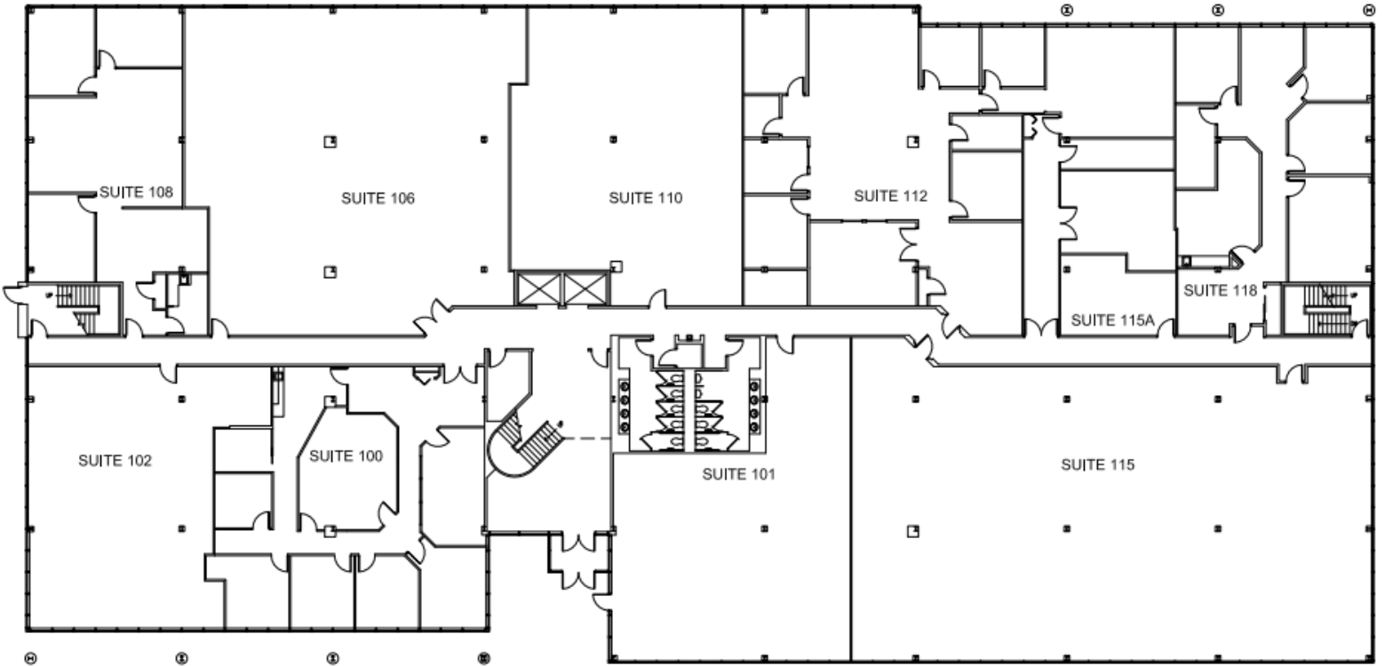
FIRST FLOOR PLAN - CORPORATE HILL ←
